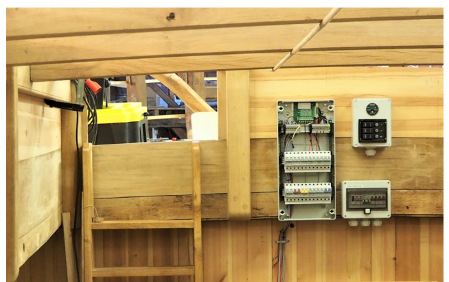
El- installation
